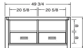
MISS BTV 2050 2 TIROIRS / 2 DRAWERS
