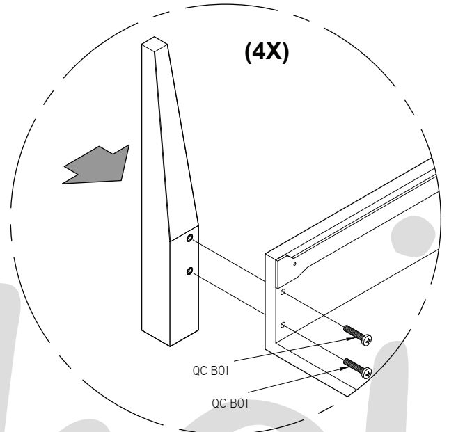
DETAIL A
