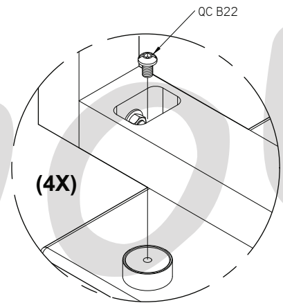
DETAIL B
